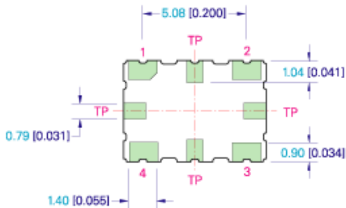
BOTTOM VIEW
