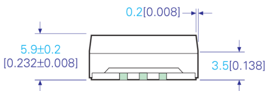
SIDE VIEW (6 PAD)
