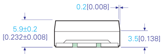
SIDE VIEW (4 PAD)
